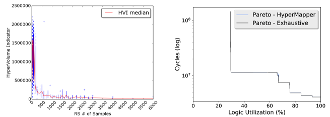
(a) HyperMapper HVI versus initial number of random samples ( R ) (b) Exhaustive and HyperMapper ( R=1000 ) generated Pareto curves.
